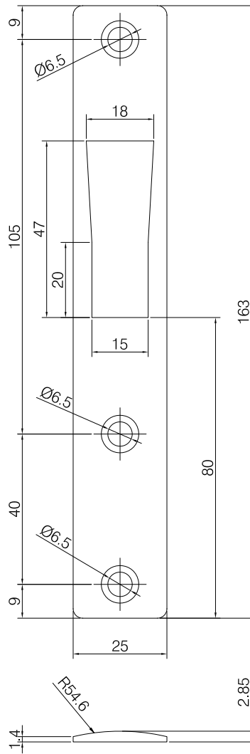
LK-1800-51-R (Radiused) AXIM trim strike plate
