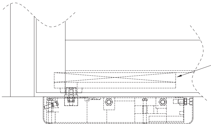
Set cement box level with finished floor level
